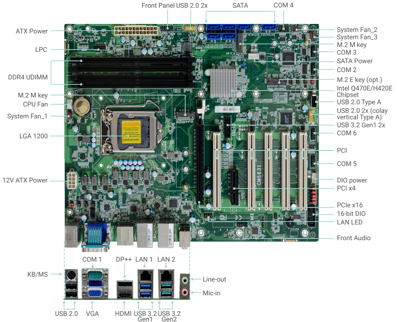
Top View
